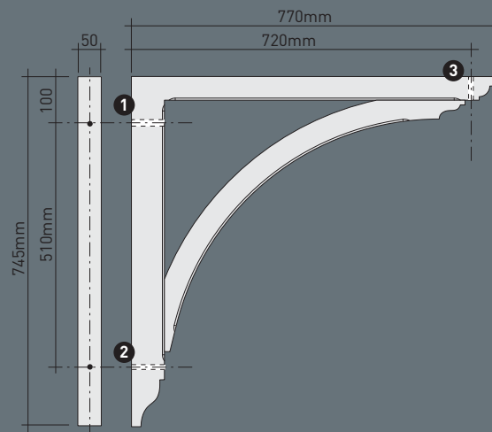
GB04 50 x 745 x 770 mm 2" x 29 5 / 16 " x 30 5 / 16 " - structural max. 75 kg* - white wood grain finish
