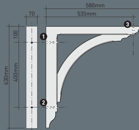
GB03 70 x 630 x 580 mm 2 3 / 4 " x 24 13 / 16 " x 22 7 / 8 " - structural max. 75 kg* - white wood grain finish
