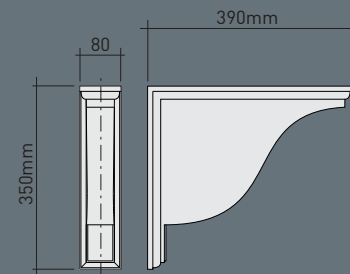
FC01 80 x 350 x 390 mm 3 5 / 32 " x 13 25 / 32 " x 15 11 / 32 "
