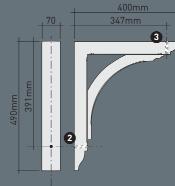
GB02 70 x 490 x 400 mm 2 3 / 4 " x 19 9 / 32 " x 15 3 / 4 " - structural max. 35 kg* - white wood grain finish
